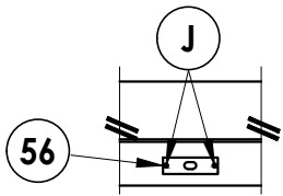
DETAIL 1 Strike Plate @ Head
