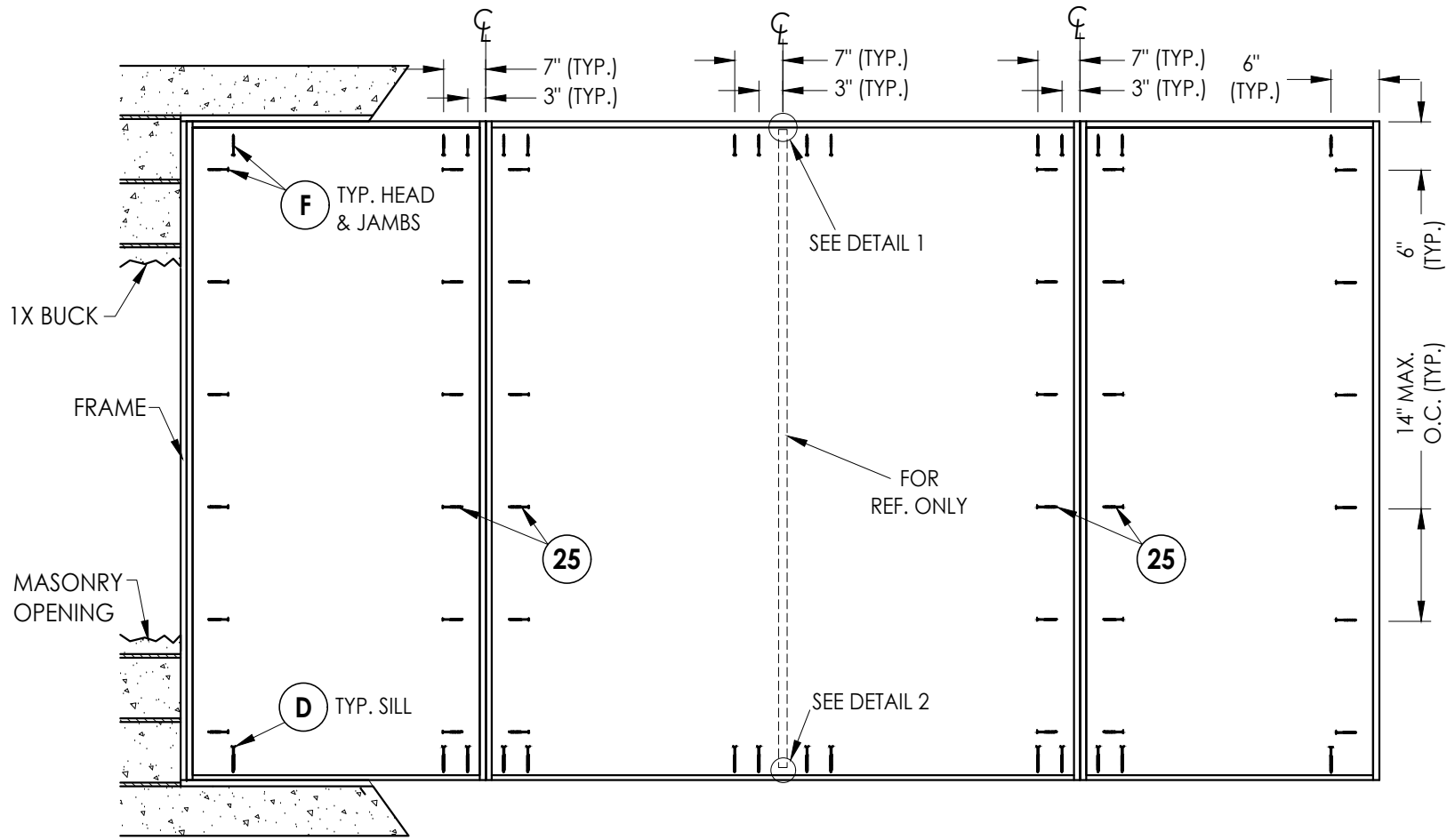
FRAME ANCHORING
