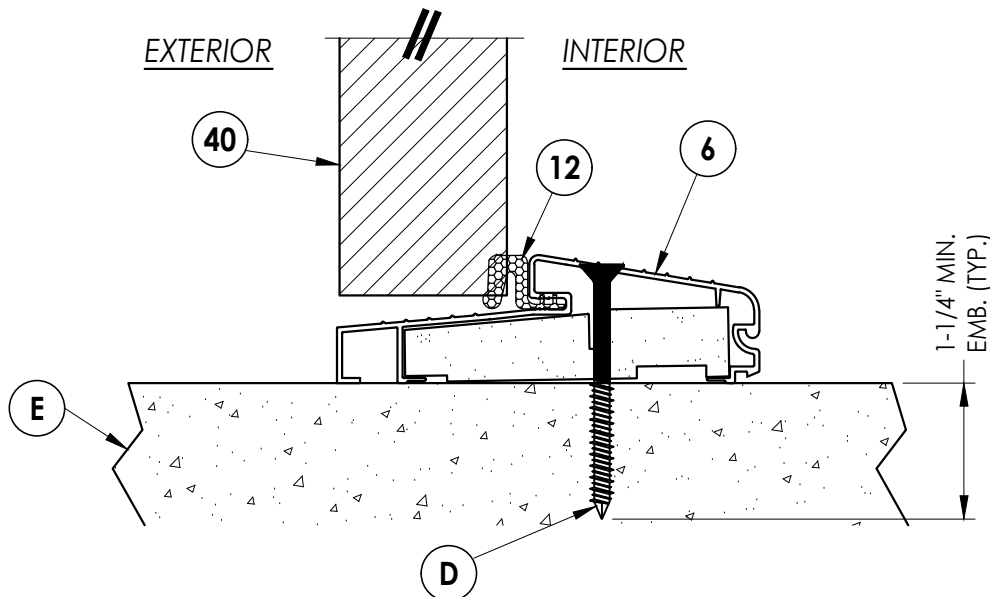
3 VERTICAL CROSS SECTION 5 Outswing sill
