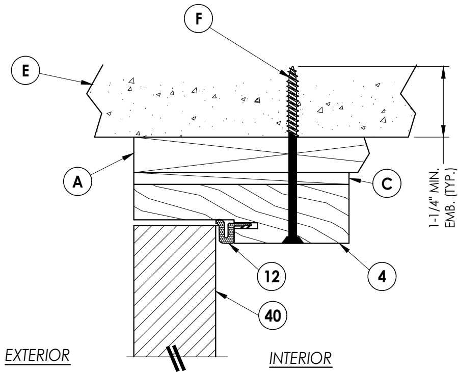
2 VERTICAL CROSS SECTION 5 Shown w/ 1X sub-buck
