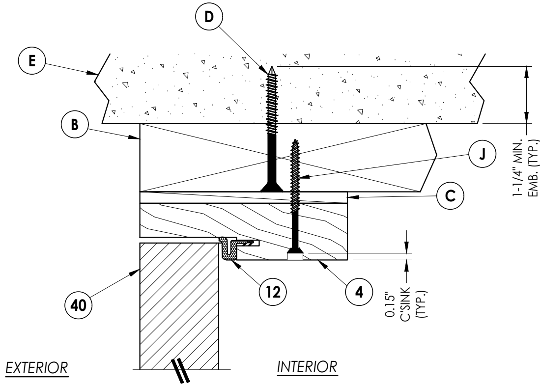
1 5 VERTICAL CROSS SECTION
