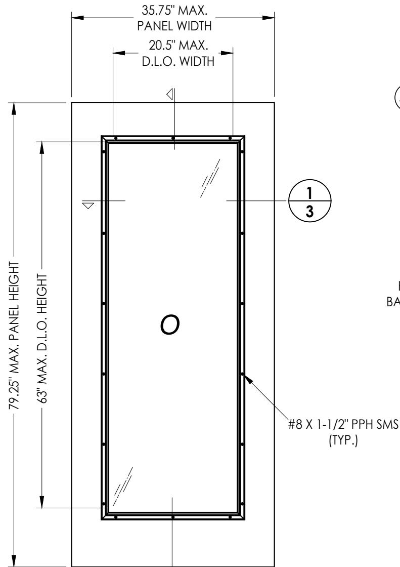
2 3 SIDELITE PANEL
