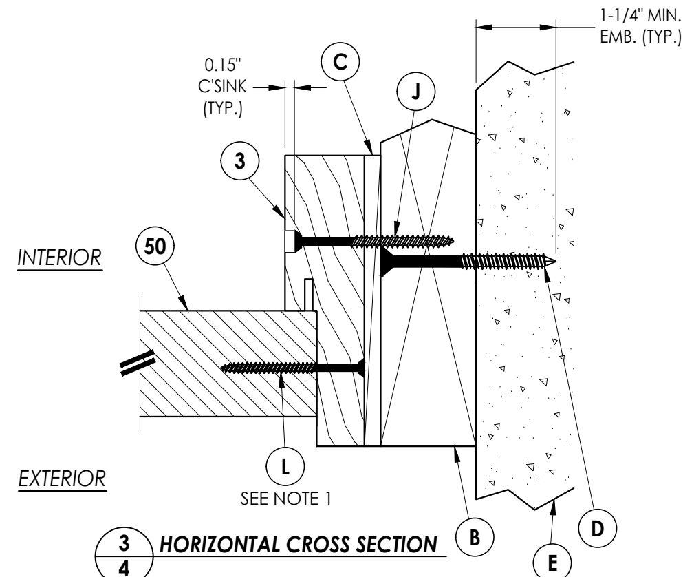
4 HORIZONTAL CROSS SECTION Shown w/ 1X sub-buck
