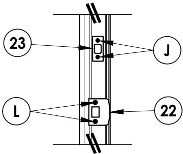
ASTRAGAL STRIKE DETAIL
