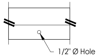
DETAIL 2 Shootbolt Hole @ Sill (Outswing)
