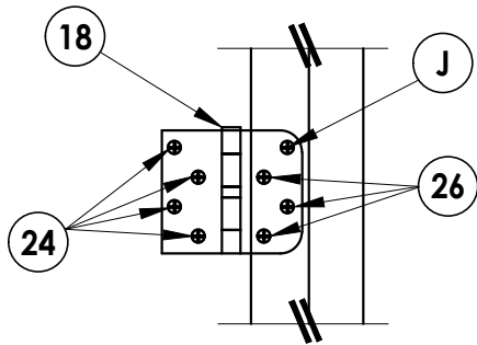
HINGE DETAIL
